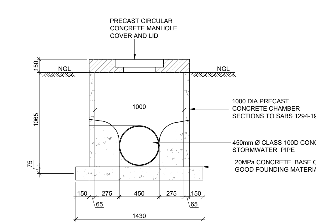
1:25 SECTION H-H
