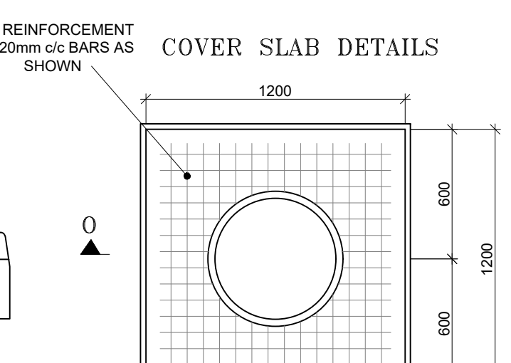
1:25 PLAN VIEW
