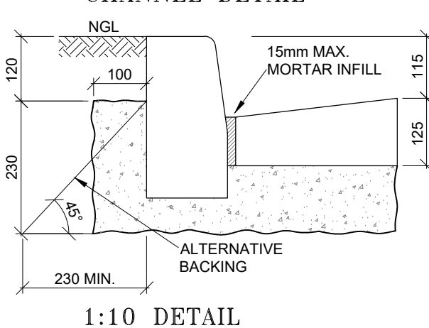
FIG. 4 KERB WITH FIG.14 CHANNEL DETAIL
