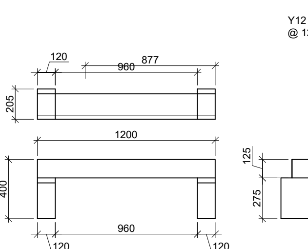
1:25 SECTION K-K
