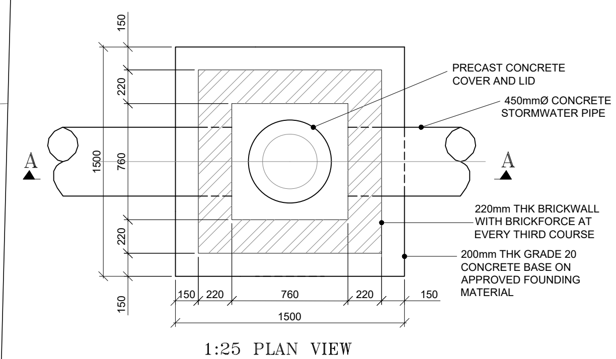
1:25 PLAN VIEW
