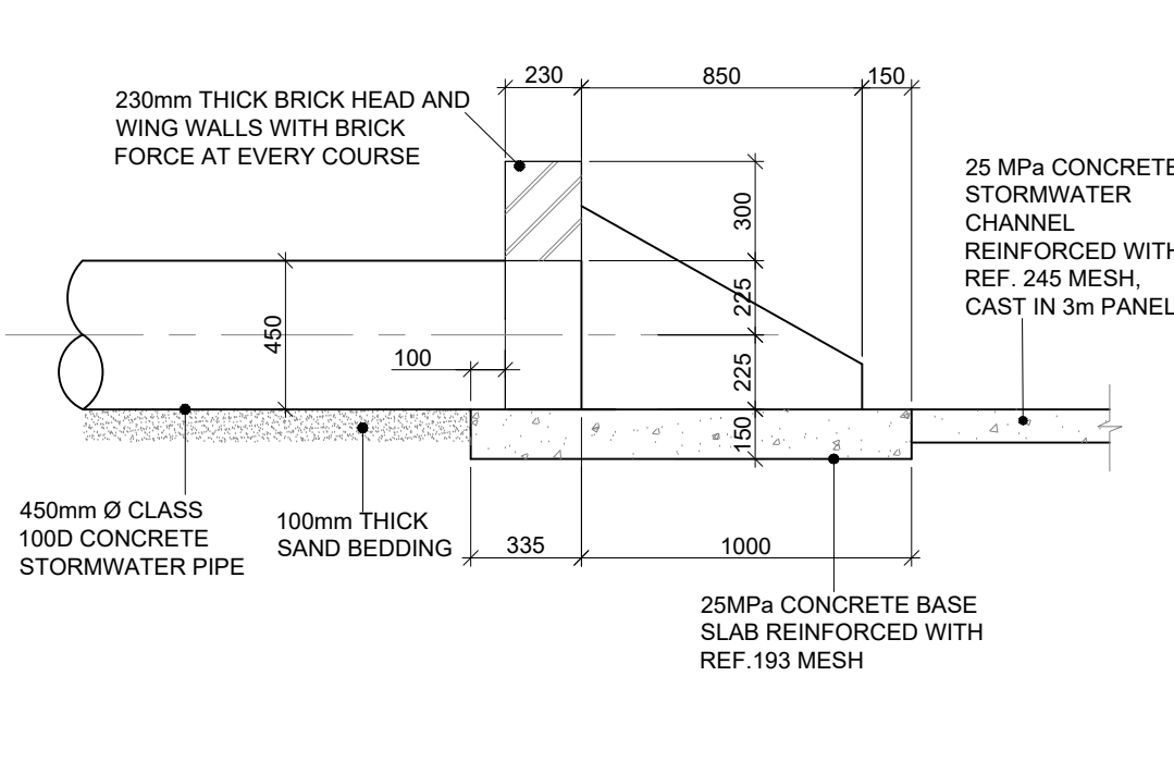
1:25 SECTION C-C
