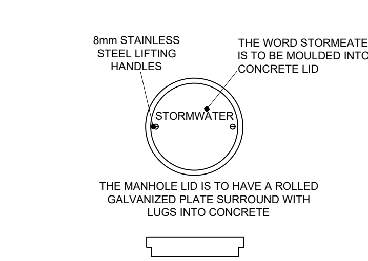
1:25 SECTION O-O
